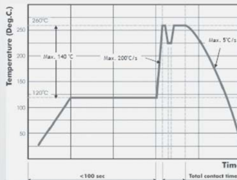
Fig. 2 Recommended wave soldering profile for SMT process with SnAgCu series solder.
