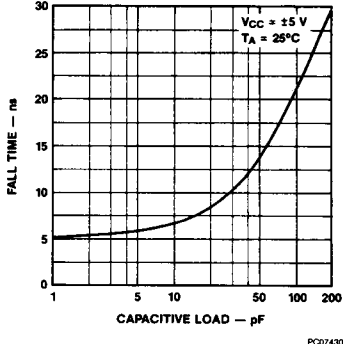
Fall Time vs Capacitive Load
