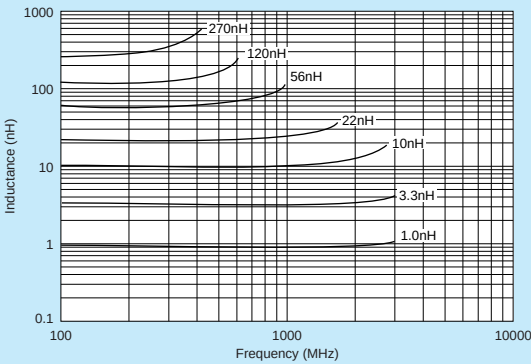
■ Inductance-Frequency Characteristics (Typ.)
