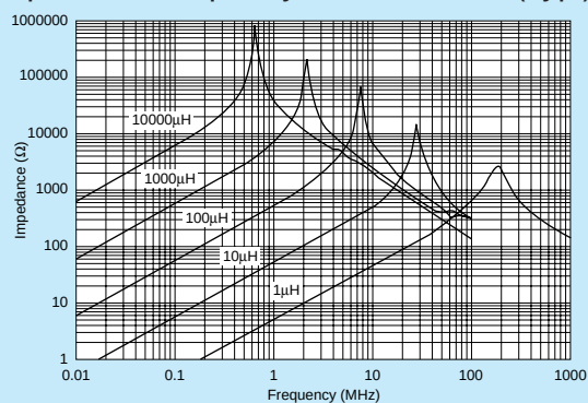
■ Impedance-Frequency Characteristics (Typ.)
