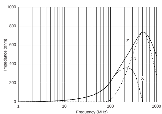
BLA2ABB221SN4
