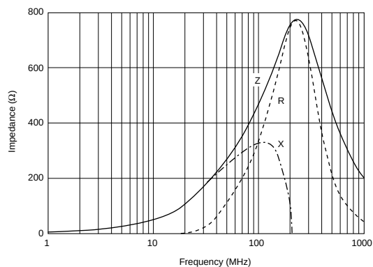
BLA31BD471SN4
