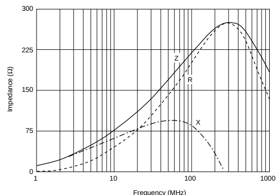
BLA31AG221SN4
