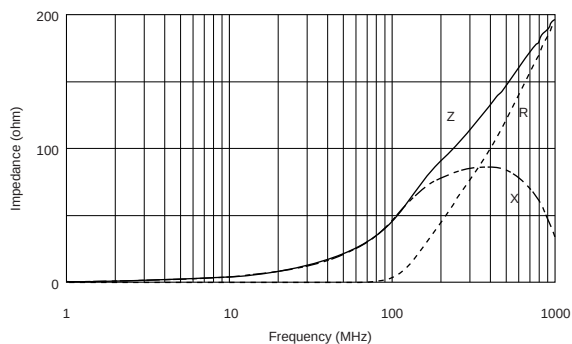
BLA2ABB470SN4
