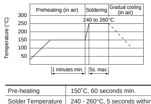
[Flow Soldering]
