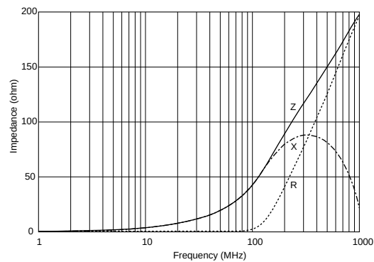
BLM15BB470SN1
