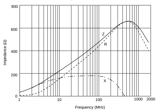
BLM18HK471SN1
