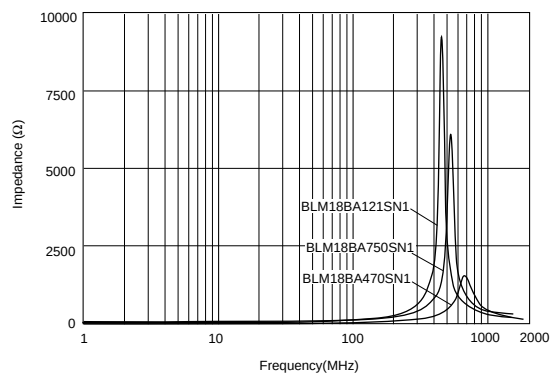
BLM18BA Series
