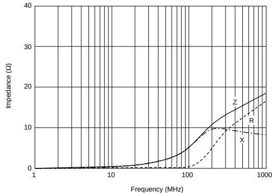
BLM18BB050SN1
