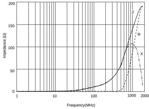
BLM18BA100SN1
