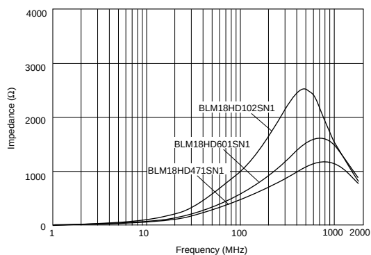
BLM18HD Series
