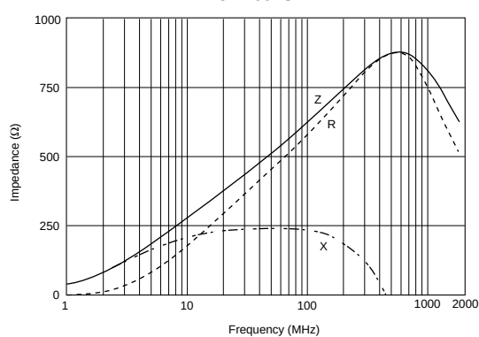
BLM18HK601SN1
