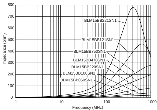
BLM15BB Series
