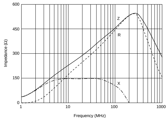
BLM18RK471SN1
