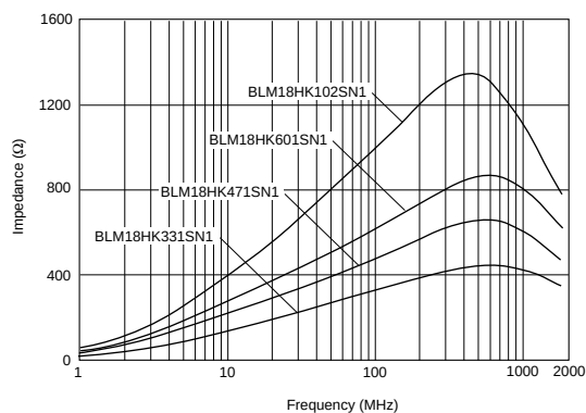
BLM18HK Series
