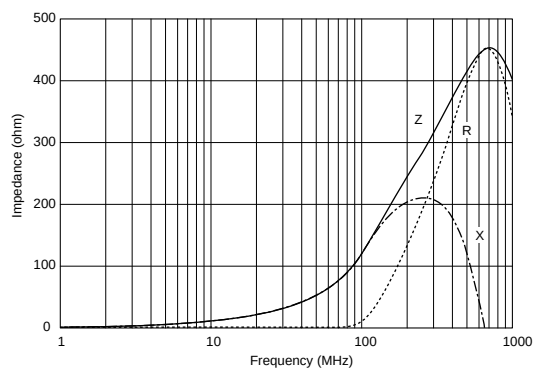
BLA2ABB121SN4
