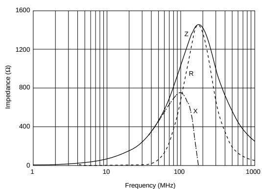
BLM15BD102SN1
