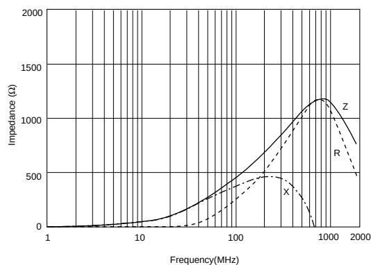
BLM18HD471SN1
