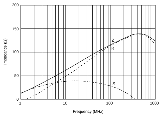
BLM18RK121SN1
