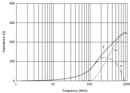
BLM18BB600SN1
