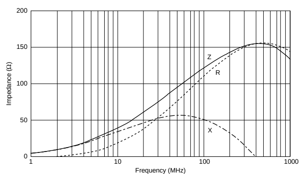
BLM18PG121SN1
