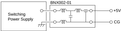
[Testing Circuit]
