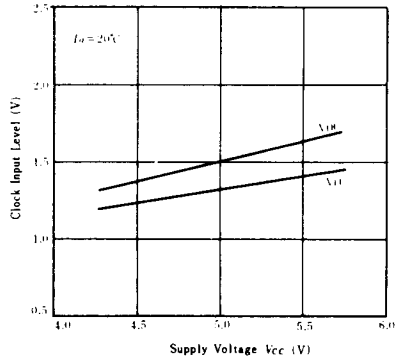
CLOCK INPUT LEVEL vs. SUPPLY VOLTAGE
