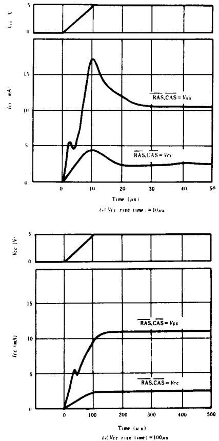
Fig.1 I_{CC} vs. V_{CC} during power up.
