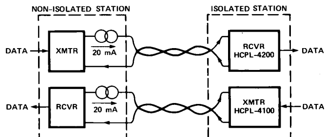
Figure 21. Full Duplex Point-to-Point Current Loop System Configuration.
