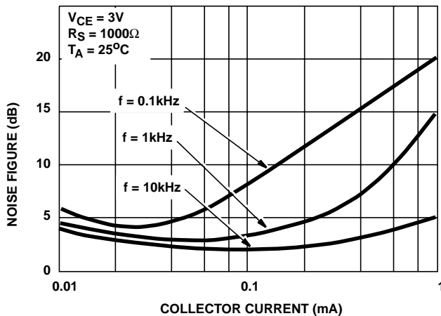
FIGURE 11. NOISE FIGURE vs COLLECTOR CURRENT
