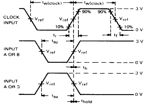
SWITCHING TIMES VOLTAGE WAVEFORMS
