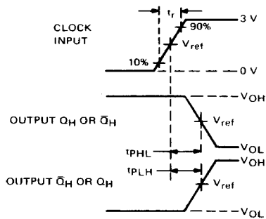
PROPAGATION DELAY TIMES VOLTAGE WAVEFORMS
