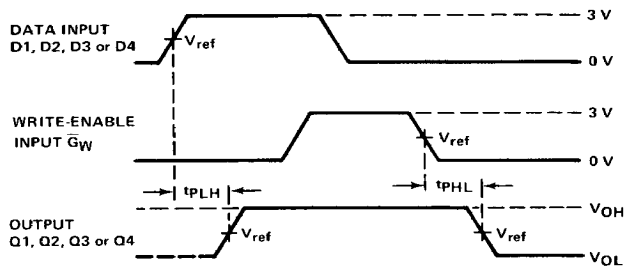
VOLTAGE WAVEFORM 1
