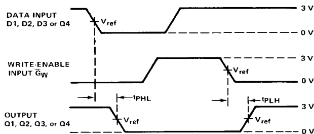
VOLTAGE WAVEFORM 2
