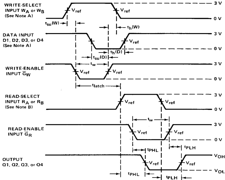
VOLTAGE WAVEFORMS
